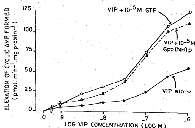
Fig. 3. Dose-response curves of adenylate cyclase activity stimulated by natural VIP, in the absence (●—●) or in the presence of 10 -5 M GTP (○—○) or 10 -5 M Gpp(NH)p (△—△) in an adenopituitary particulate fraction. This fraction was the resuspended 4000 × g pellet obtained after centrifugation of the 180 × g supernatant of an adenopituitary homogenate from male rats. The dose-effect curves were the means of 4 expt performed in duplicate. The results were expressed in pmol cyclic AMP formed · min -1 · mg protein -1 in excess of the corresponding control values, i.e., 33, 74 and 172 pmol cyclic AMP · min -1 · mg protein -1 formed, respectively, in the absence of any addition, and in the presence of 10 -5 M GTP or 10 -5 M Gpp(NH)p. The values found in the presence of nucleotides were significantly higher than those observed in the absence of nucleotides ( p < 0.001 based on Student's t test for paired values).
